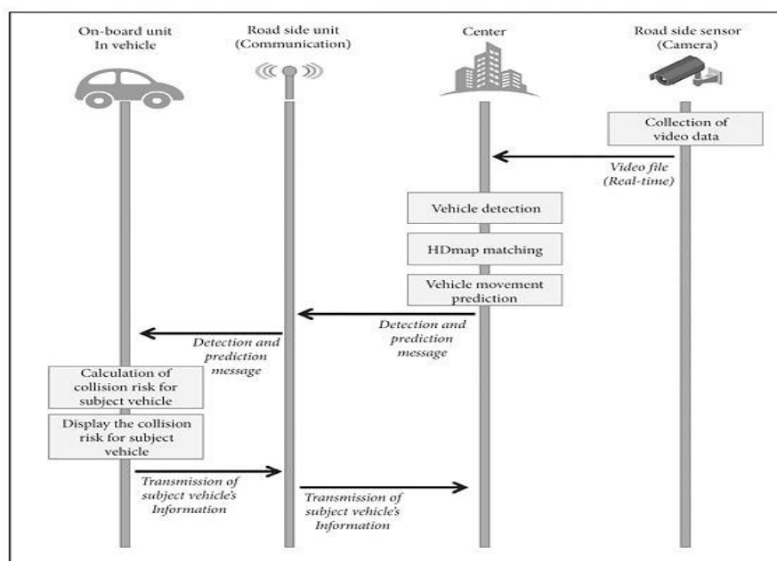
Fig. 3. Data flow in smart traffic management with edge computing.
